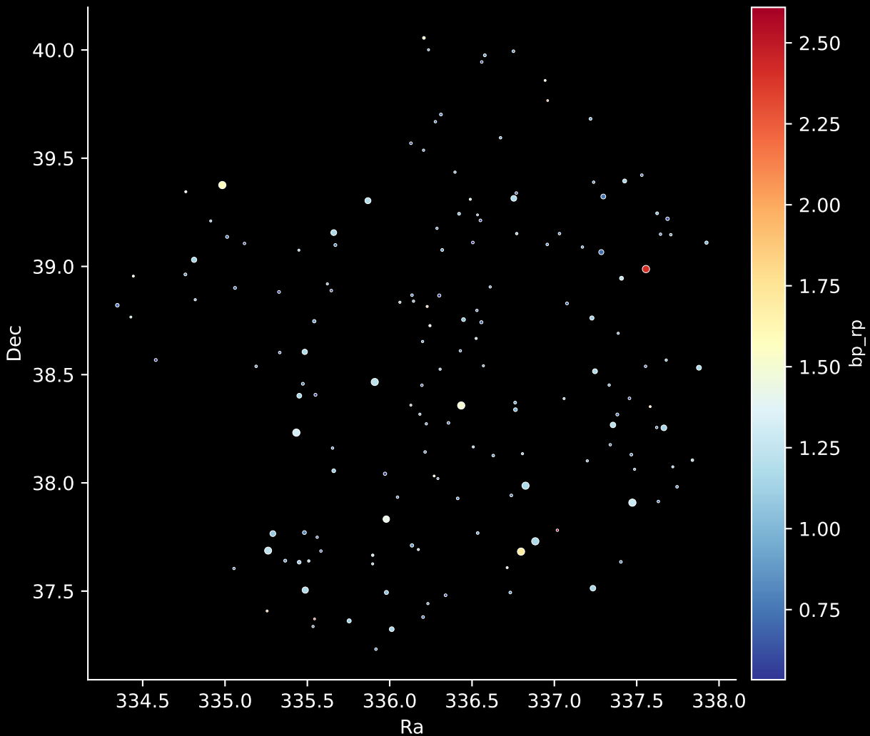
APOGEE DR17 Field: [062+52_MGA] Stars: 161
