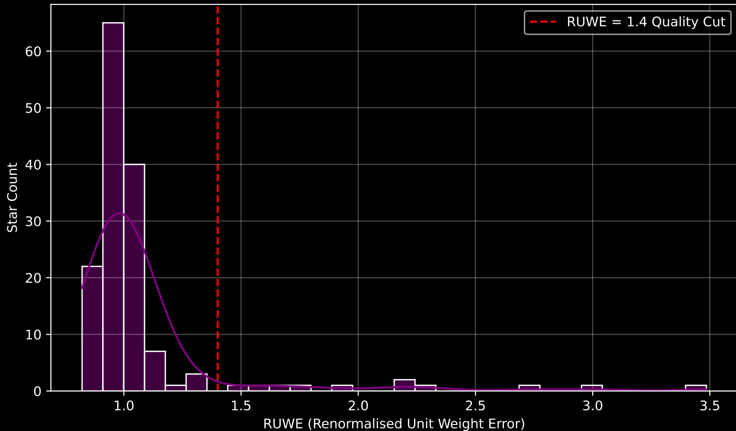
GAPOGEE DR17 Field [062+52_MGA] RUWE Distribution (n= 149)
