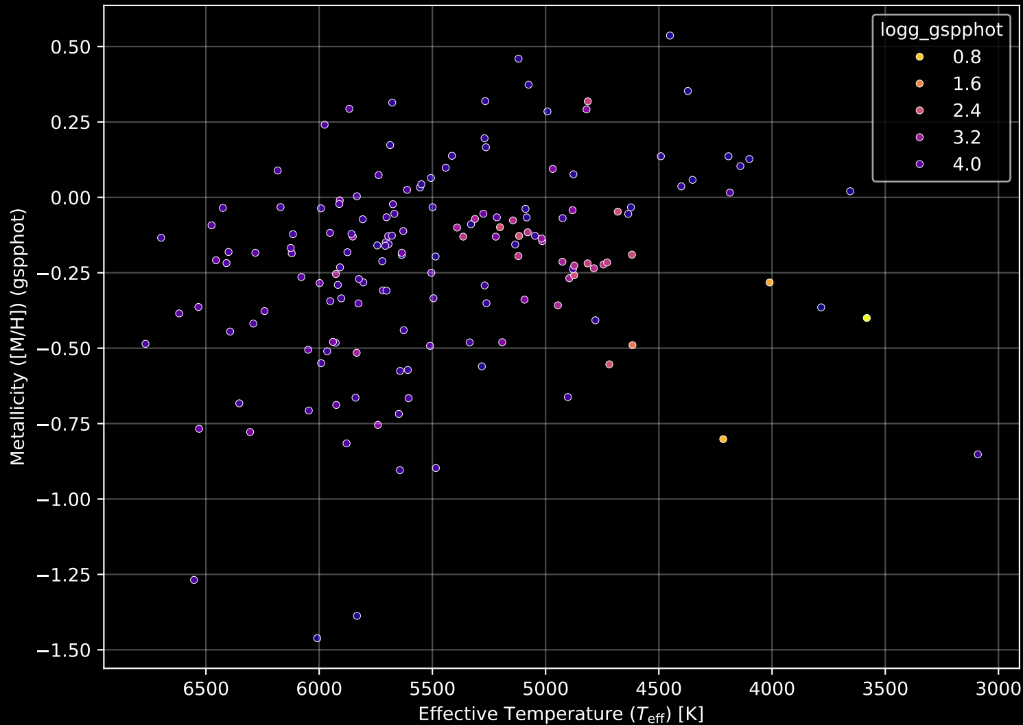
APOGEE DR17 Field: [062+52_MGA] Stellar Population Parameters (n= 161)
