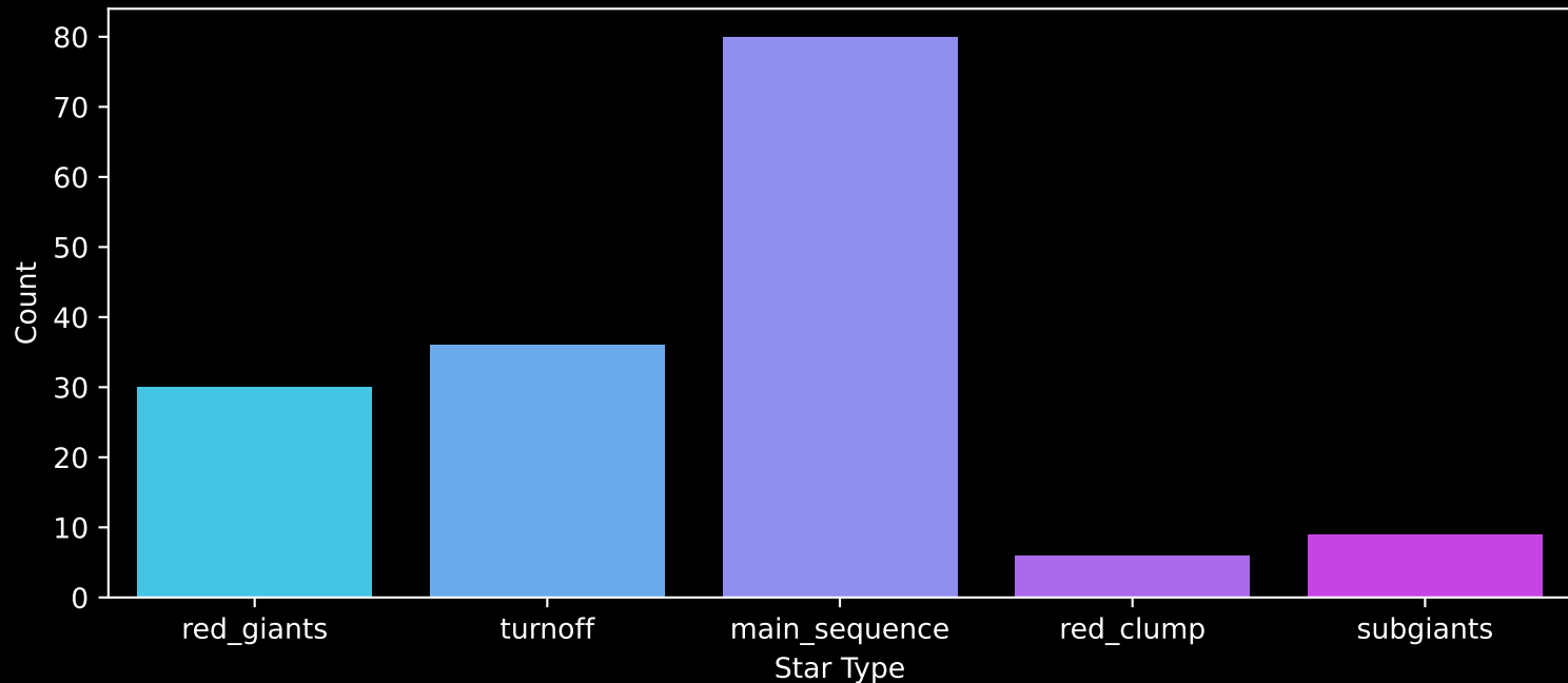
APOGEE DR17 Field: [062+52_MGA] Count plot of Star Type
