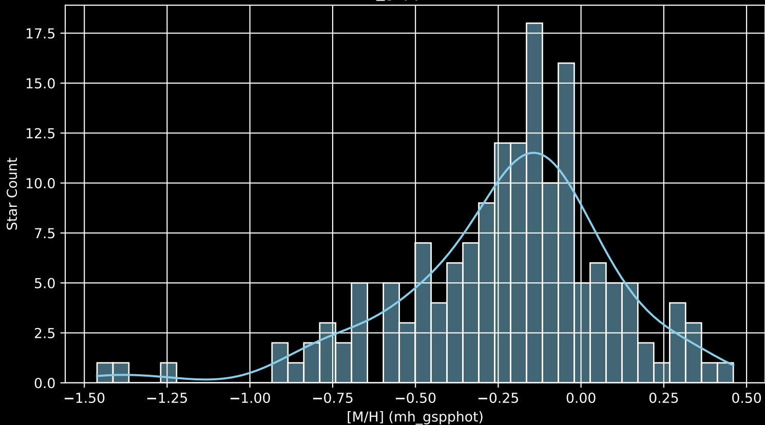
APOGEE DR17 Field: [062+52_MGA [M/H] (mh_gspphot) (n= 160)
