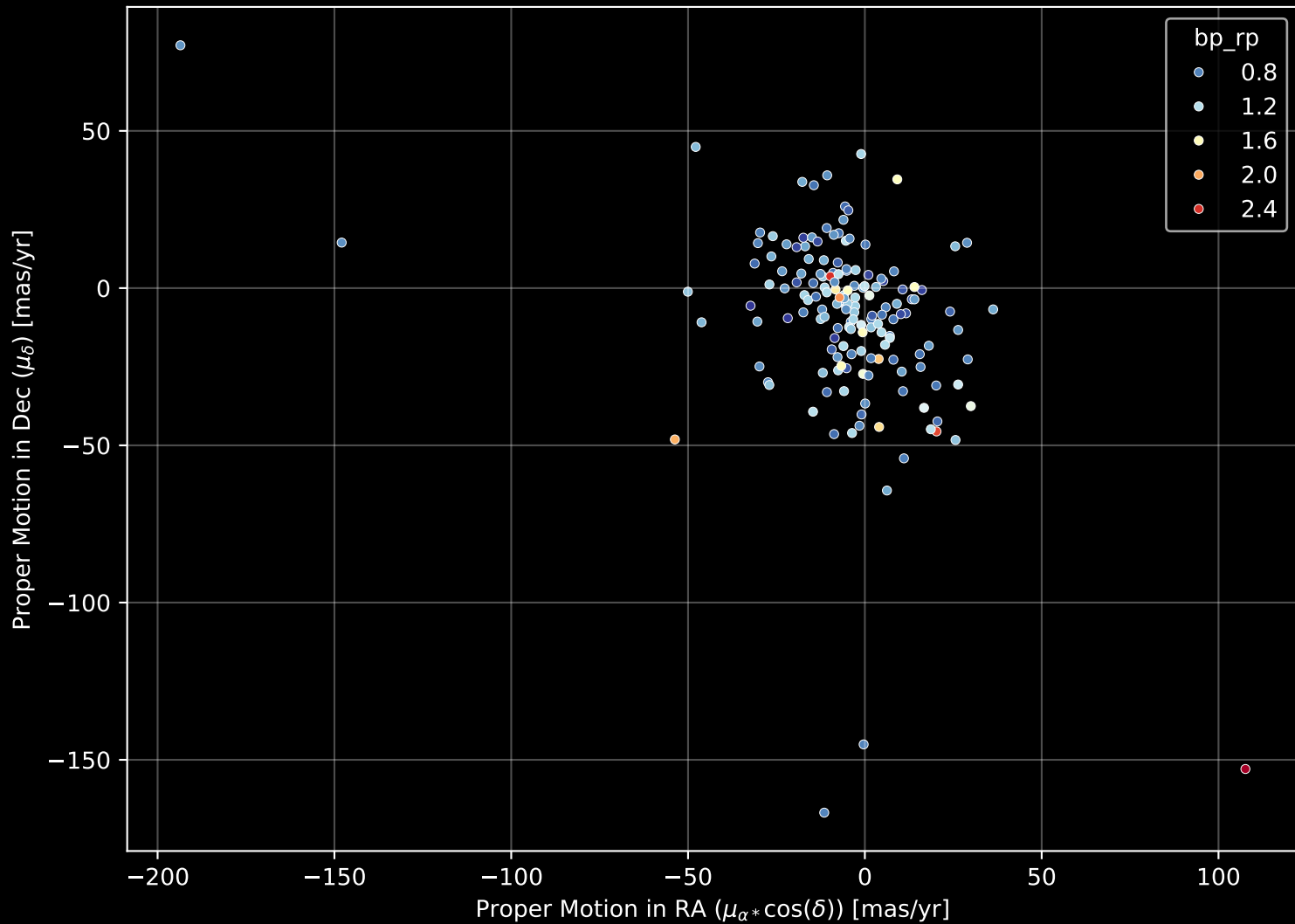
APOGEE DR17 Field: [062+52_MGA] Proper Motion Diagram (n= 161)
