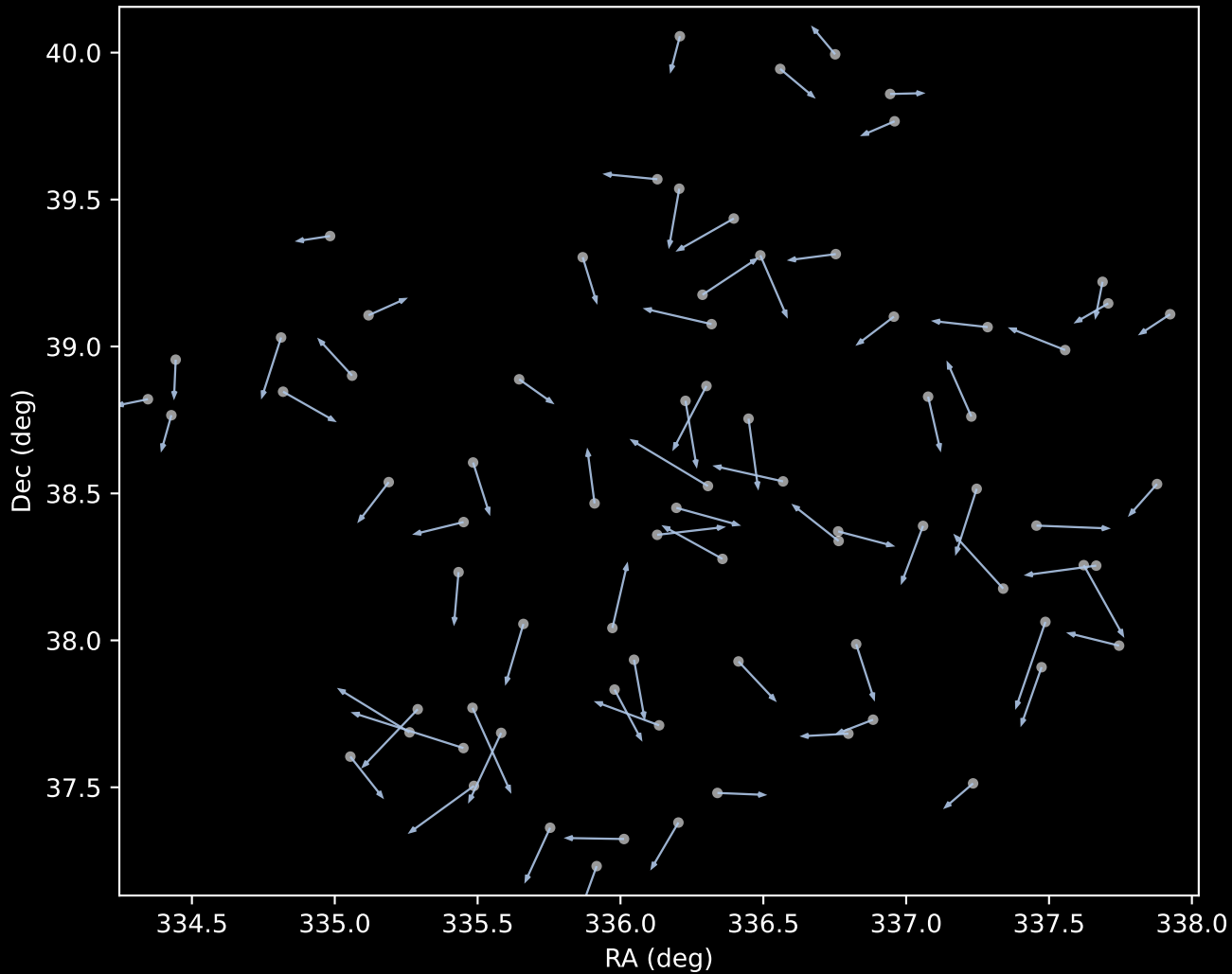
APOGEE DR17 Cluster 1 Proper Motion Vectors (n=77)
