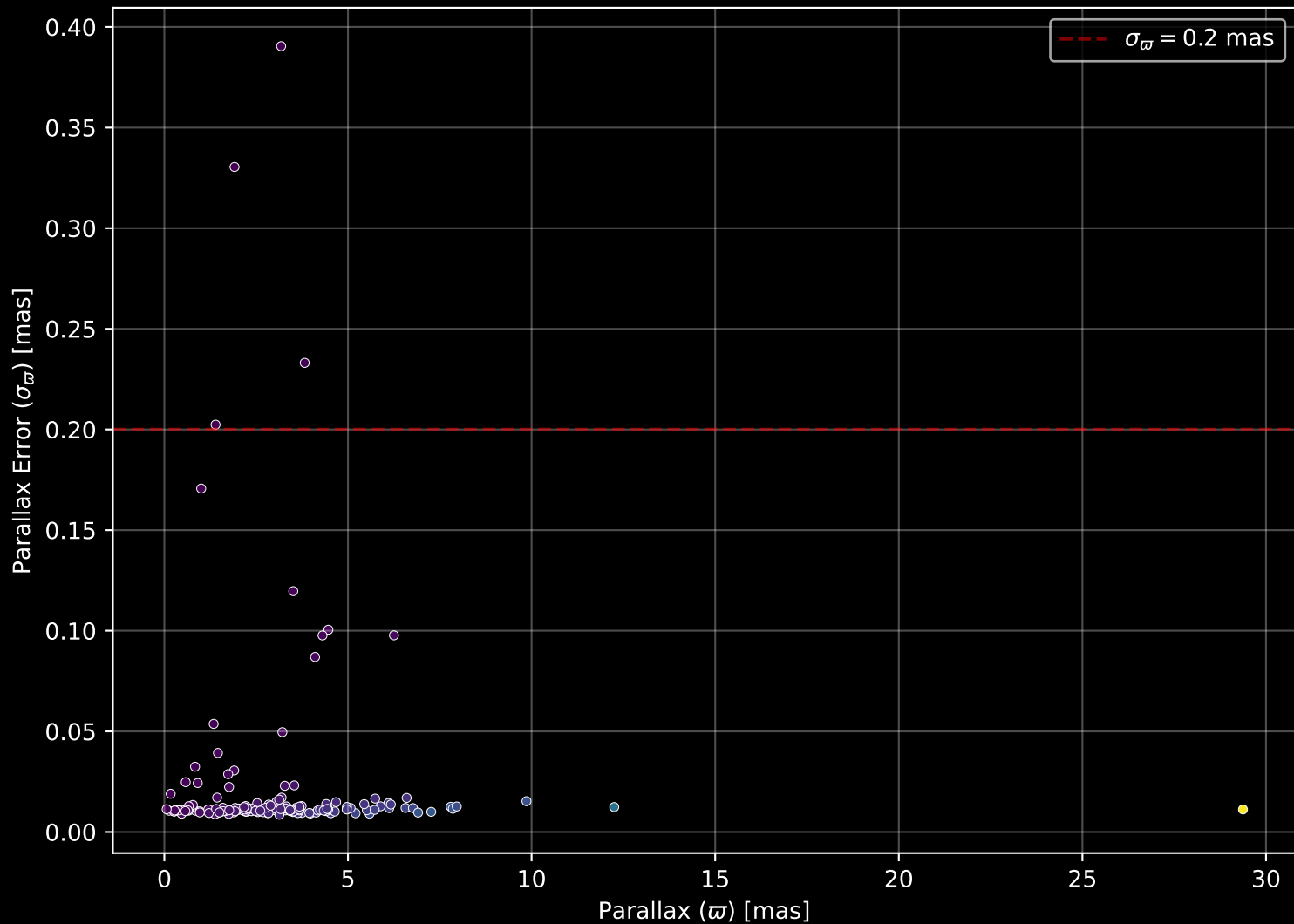
APOGEE DR17 Field: [062+52_MGA] Parallax Quality (n= 161)
